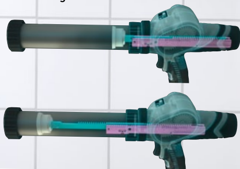
Double rack system for compact tool design
