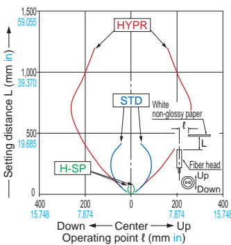
FD-S60Y
