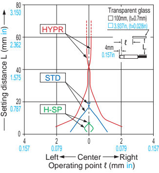
FD-H25-L43
