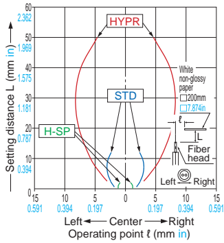
FD-EG30S
